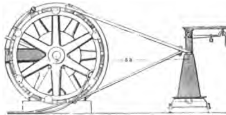
FIG. 310a. —Common Form of Prony Brake, for testing the D. H. P. of an engine. An iron band shod with wooden blocks is drawn tightly around the circumference of the fly-wheel. To this two arms are attached, the other ends of which bear upon the scale platform, as shown. It is necessary that the scale platform be raised to the same height as the centre of the fly-wheel shaft. The length of leverage is indicated as 5 feet 3 inches, the diameter of the wheel being 3 feet. These two factors, the R. P. M. and the recorded weight, are the essential elements in the determination of power as by the above formula.
